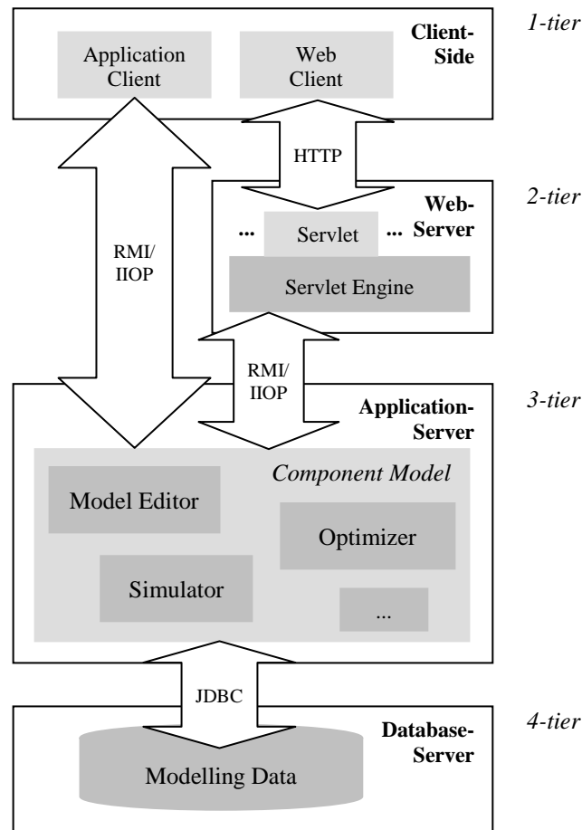
Figure 2. Possible realization of a component-oriented M&S tool based on a distributed 4-tier architecture
